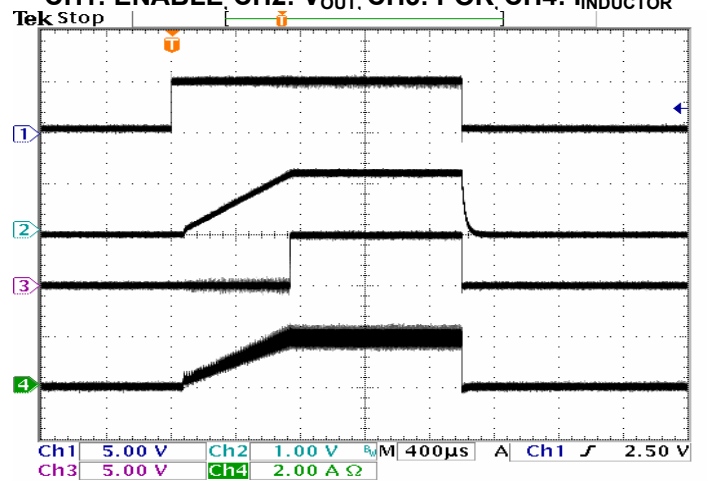
CH1: ENABLE, CH2: V_{OUT} , CH3: POK, CH4: I_{INDUCTOR}
