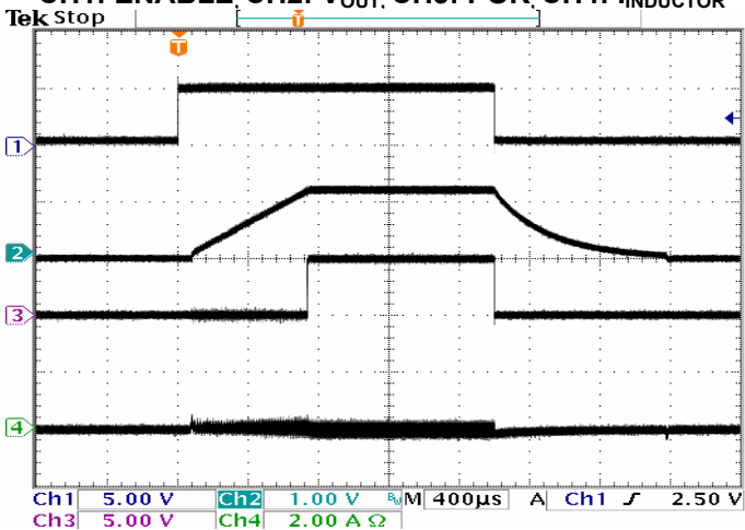
CH1: ENABLE, CH2: V_{OUT} , CH3: POK, CH4: I_{INDUCTOR}
