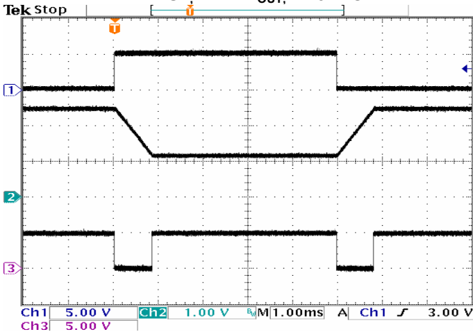
Power Up/Down at No Load ( V_{IN} = 5\text{ V} , V_{OUT} = 1.2\text{ V} )
