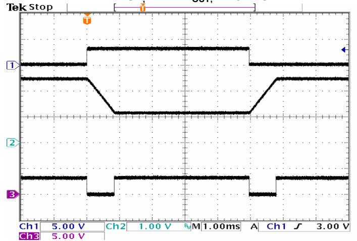
Power Up/Down at 0.6\ \Omega Load ( V_{IN} = 5\text{ V} , V_{OUT} = 1.2\text{ V} )
