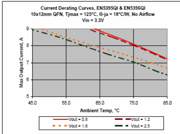
Figure 6 . Output Current Derating Curve, V_{IN} = 3.3V
