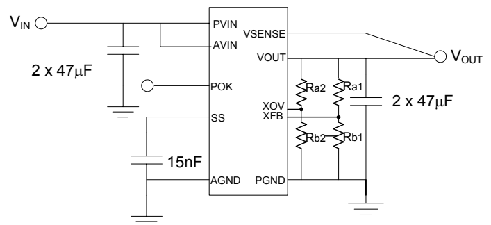
Figure 4. V_{OUT} and OVP resistor divider networks.
