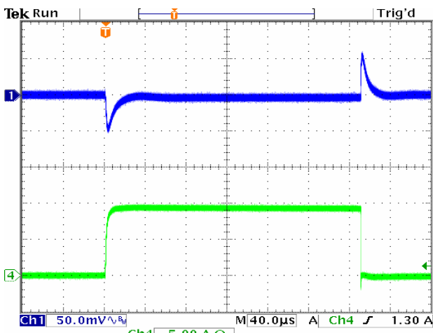
Transient Response: 5V_{IN}/1.2V_{OUT} , 0\text{-}9\text{A} , 7\mu\text{s} . C_{OUT} = 5 \times 22\mu\text{F} .
