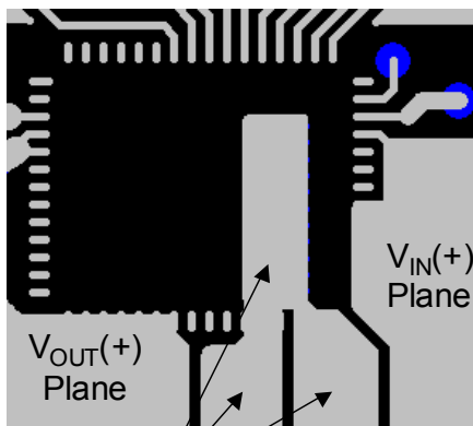
Figure 7. Layout of power and ground planes.
