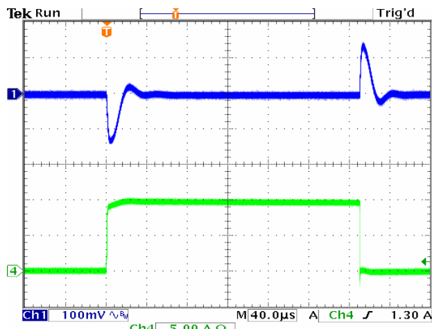
Transient Response: 5V_{IN}/3.3V_{OUT} , 0\text{-}9\text{A} , 7\mu\text{s} . C_{OUT} = 5 \times 22\mu\text{F} .
